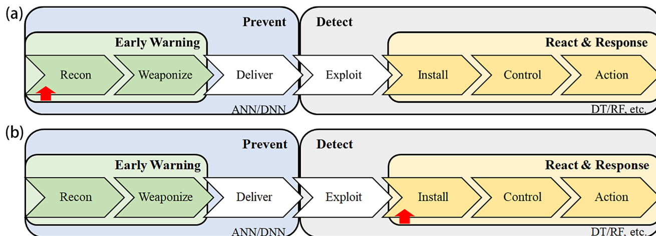
Fig. 1 Process of using AI and Shadow AI use in an organization. (a) Using an authorised AI module in an organization; the processes are aware to the organization from the arrow mark. (b) Using a Shadow AI
