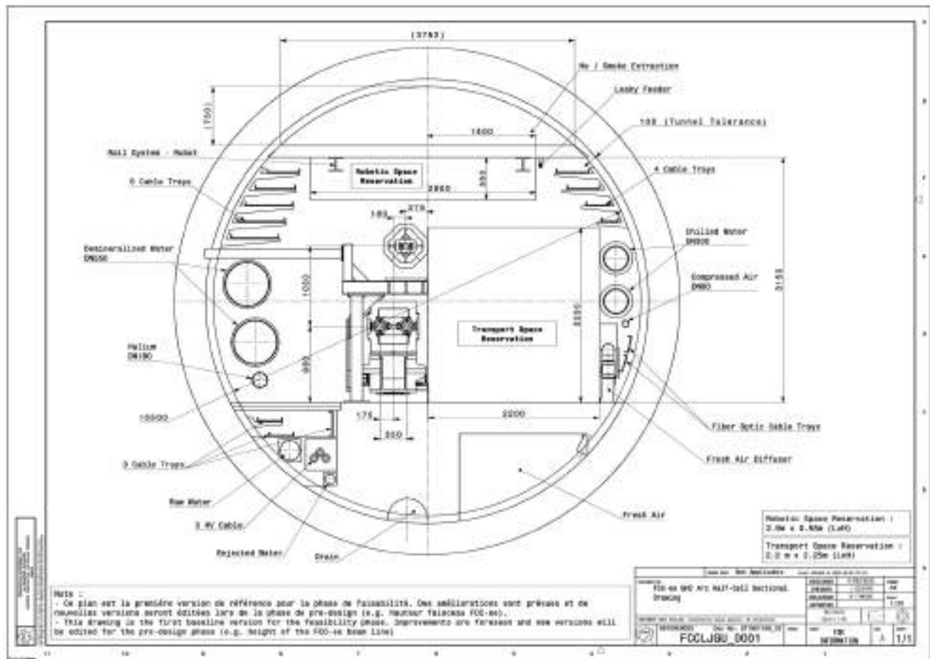
Fig. 3.71 FCC-ee GHC Arc Half-Cell sectional drawing - EDMS 3180552 [319]
