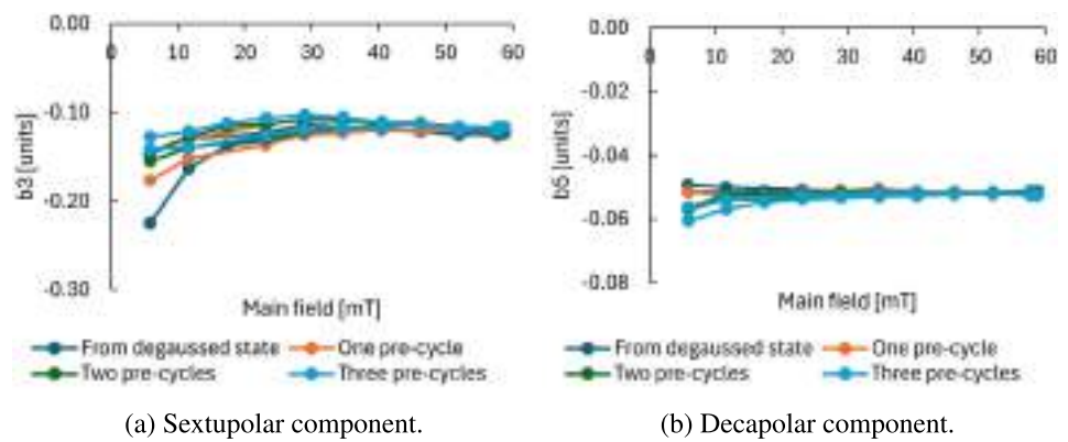
Fig. 6.3 2D field harmonics in the short prototype booster dipole at the t\bar{t} field levels. Values quoted at R = 10 mm in units of 1 \times 10^{-4} [342]
