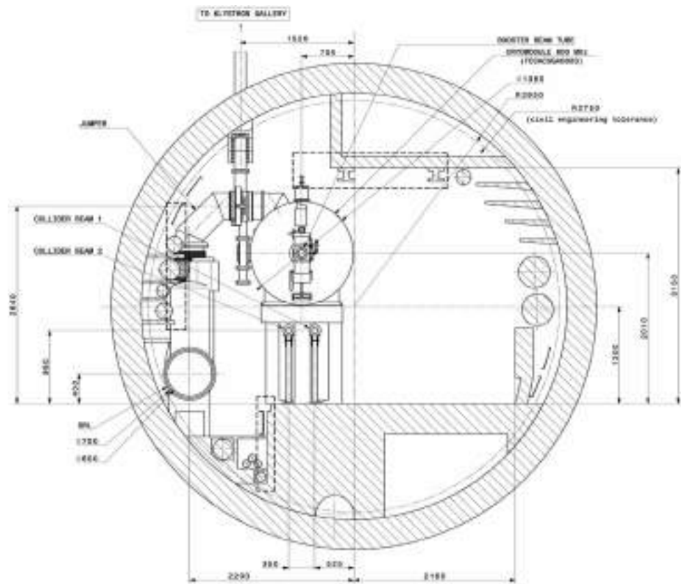
Fig. 3.46 800 MHz cryomodule, integration in point PL (booster)
