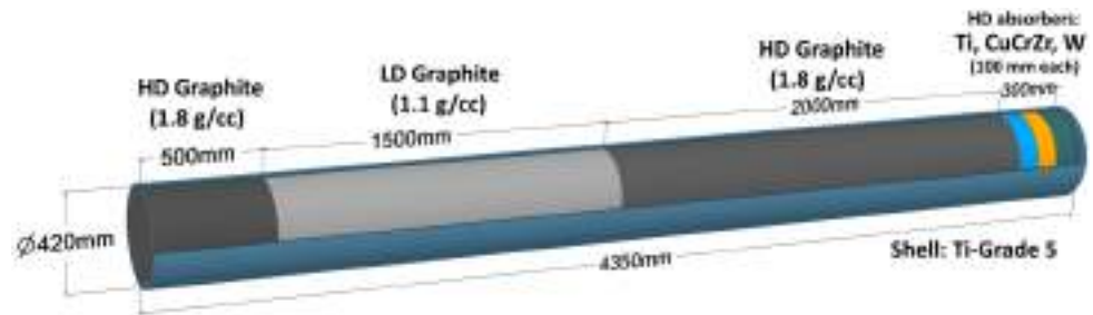
Fig. 3.52 Schematic diagram of the FCC-ee dump block design, showing the material for the dump core and the vessel
