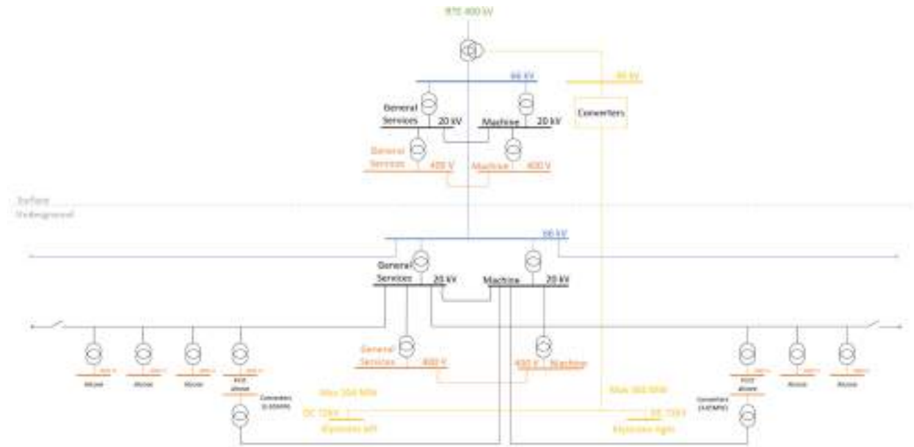
Fig. 3.60 Concept of electrical distribution at point PH
