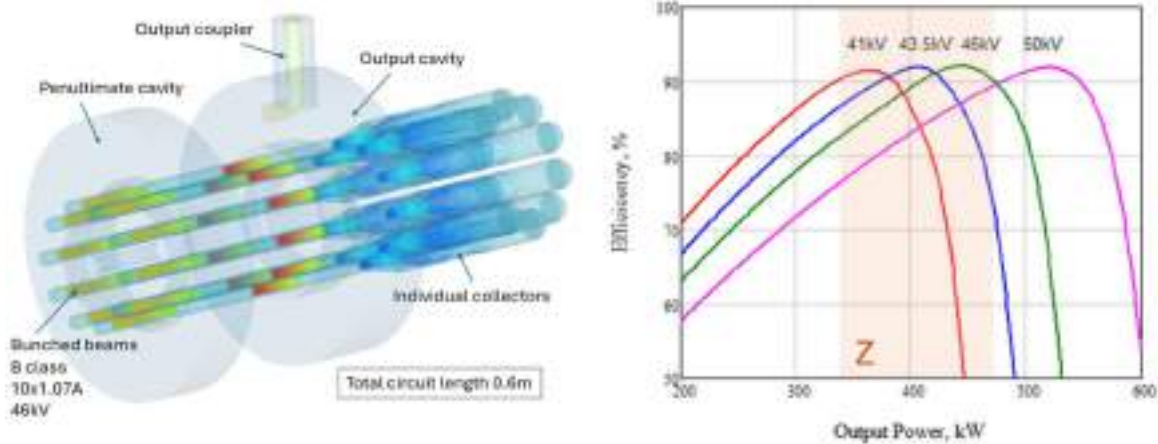
Fig. 3.40 Left: A snapshot of particle dynamics in the tristrion simulated in 3D PIC CST. Right: RF power/efficiency performance at different operating voltages
