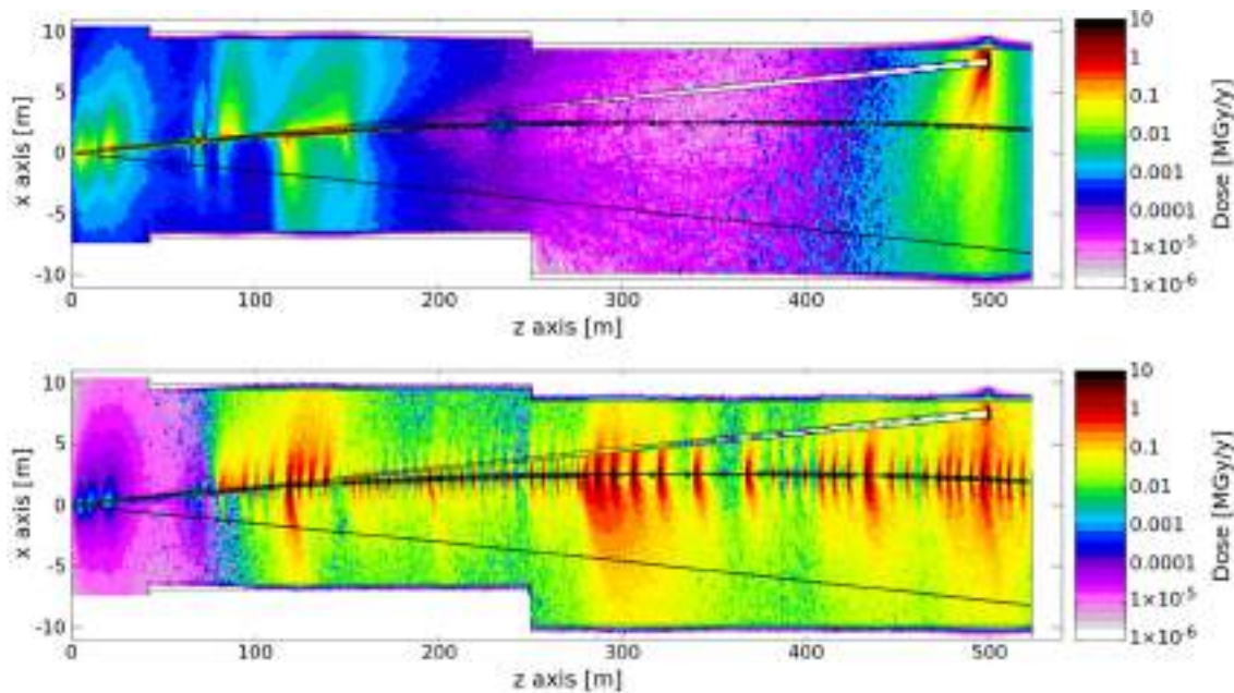
Fig. 1.43 Top view of the annual ionising dose at the beamline level (average for y in [-20, 20] cm) caused by beamstrahlung radiation, radiative Bhabha electrons and synchrotron radiation from the outgoing beam. The top figure corresponds to Z mode operation, whereas the bottom figure is for t\bar{t} . The maps were simulated with FLUKA
