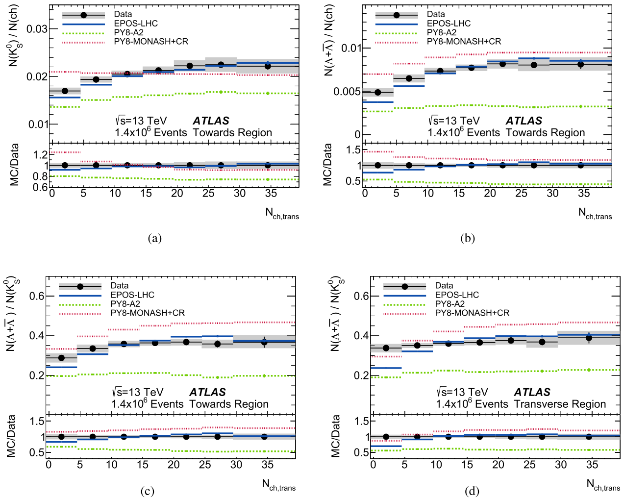
Fig. 7 Comparison between data and MC simulation for several multiplicity ratios as a function of N_{ch,trans} in events with leading jet 10 < p_T \leq 40 GeV. Shown are the prompt charged-particle normalised a K_S^0 and b (\Lambda + \bar{\Lambda}) multiplicity yields in the towards region,
