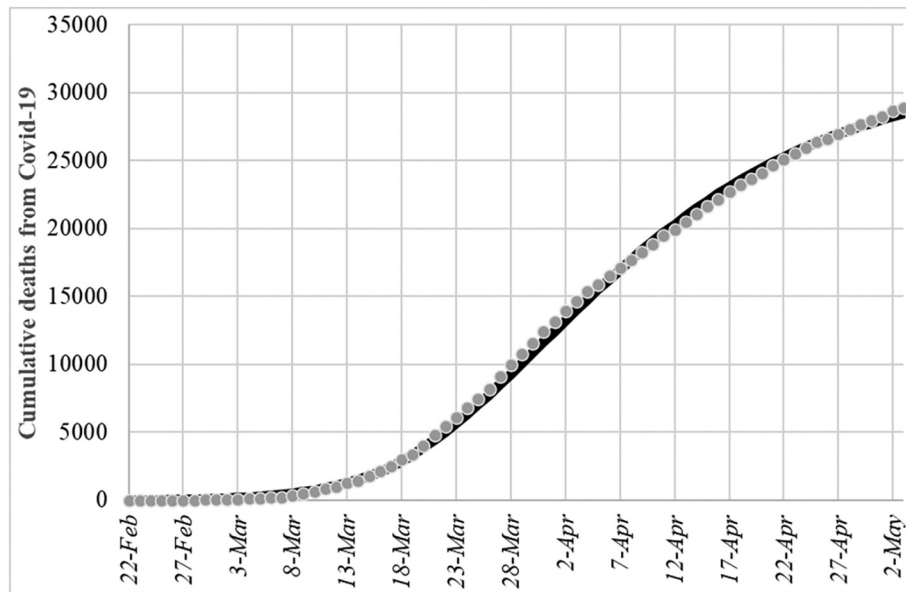
Fig. 2. Predicted evolution of the cumulative number of Covid-19 deaths in Italy, black curve fitted to real data points in grey (up to May 3rd).
