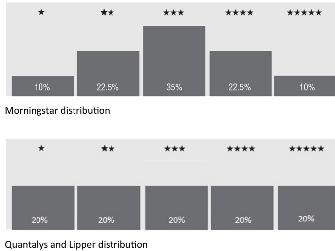
Fig. 2. Distribution of ordinal measures and rating assignment.
