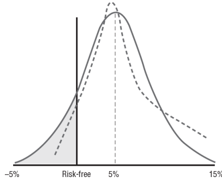
Fig. 1. Standard deviation, downside risk and return distribution.
