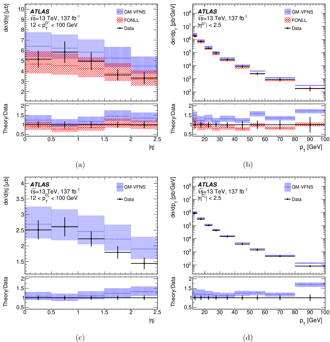
Figure 8. Differential cross-sections for D^\pm mesons in bins of (a) |\eta| and (b) p_T , and for D_s^\pm mesons in bins of (c) |\eta| and (d) p_T . The measured values with the statistical and systematic uncertainty are represented by the data points, while the theory predictions from GM-VFNS and FONLL are shown as dotted and dashed lines, respectively; the uncertainties on the theory predictions are represented by the hatched areas. The theory predictions are also divided by the measured values to obtain the ratios between the predictions and the measurements shown in the bottom panels.
