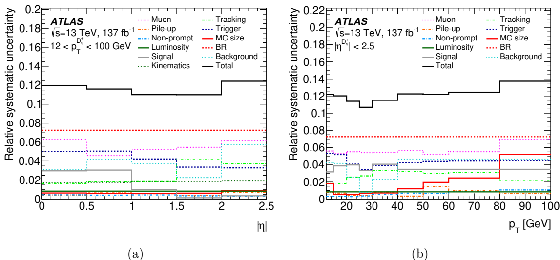
Figure 7. Relative systematic uncertainty profile of the differential cross-sections for D_s^\pm mesons, in bins of (a) |\eta| and (b) p_T . The systematic uncertainties shown are also combined in quadrature (upper solid line).
