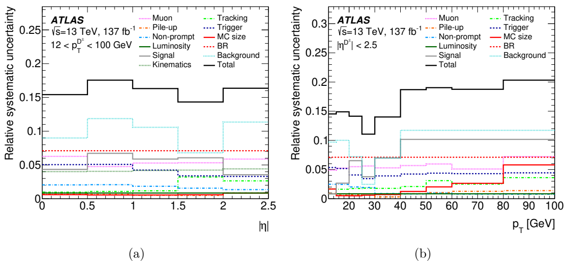
Figure 6. Relative systematic uncertainty profile of the differential cross-sections for D^\pm mesons, in bins of (a) |\eta| and (b) p_T . The systematic uncertainties shown are also combined in quadrature (upper solid line).
