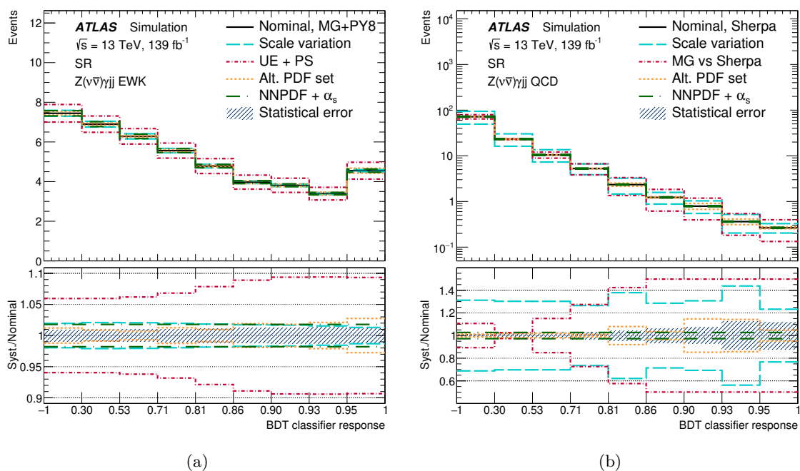
Figure 3. These graphs indicate the effect of the main theory uncertainties, which are associated with the renormalisation and factorisation scales (dashed cyan), underlying event and parton showering (UE+PS) or generator choice (dash-dotted red), alternative PDF sets (dotted orange), combined NNPDF set variation and \alpha_s uncertainty (loosely dash-dotted green). These are shown in the signal region for (a) the Z(\nu\bar{\nu})\gamma jj EWK process and (b) the Z(\nu\bar{\nu})\gamma jj QCD process. The BDT classifier response was remapped into equal width bins for better representation. The uncertainty band corresponds to the uncertainty due to the limited number of MC events.
