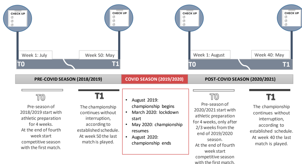
Figure 1. A timeline of the 2018–2019 and 2020–2021 Serie A seasons surrounding the impact of the COVID-19 pandemic lockdown.
