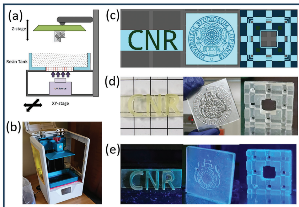
Figure 4. SLA with composite formulation \text{Cs}_4\text{PbBr}_6 (0.25)-GDRB a) SLA apparatus (with 6bottom-up configuration.) b) AnyCubic PhotonS 3D-printer c) CAD models d) 3D-printed objects before and under UV irradiation e).
