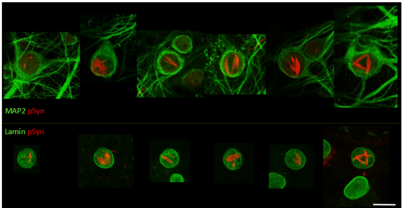
Figure 4. I-SGM optical sections of 30 DIV mouse primary cortical neurons treated at DIV7 with 1B fibrils. Phospho-S129 \alpha -Syn-positive inclusions (NIIs) are coded in red, upper row; MAP2 is in green, lower row; Lamin is in green. Scale bar: 10 \mu m.
