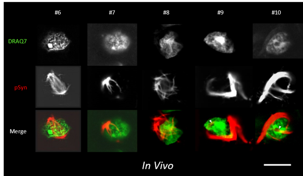
Figure 11. LSCM optical sections of the \alpha -Syn pathology spread in a mouse injected 4 months before with 1B fibrils. Phospho-S129 \alpha -Syn: coded in red; DNA/DRAQ7: coded in green. Zone injected with 1B and sampled by LSCM: right substantia nigra. Five individual nigral neurons (#6 to #10) bearing NCIs and NII are shown. For description see text. Scale bar: 10 \mu m.
