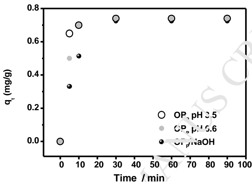
Figure 7: pH value effect on the adsorption capacity q_t (mg/g) of DB removal from aqueous ( 5 \times 10^{-5} M) solutions, at fixed OP P a.t. amount (0.25g).
