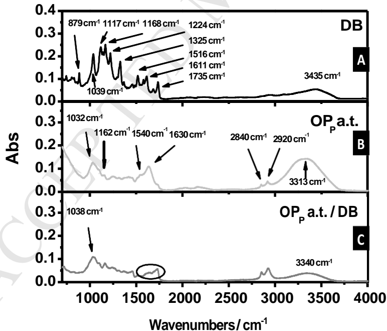
Figure 4: FTIR-ATR spectra in the range: 600-4000 \text{cm}^{-1} of DB (A); of OP P a.t. (B) and of OP P a.t./DB composite material (C).
